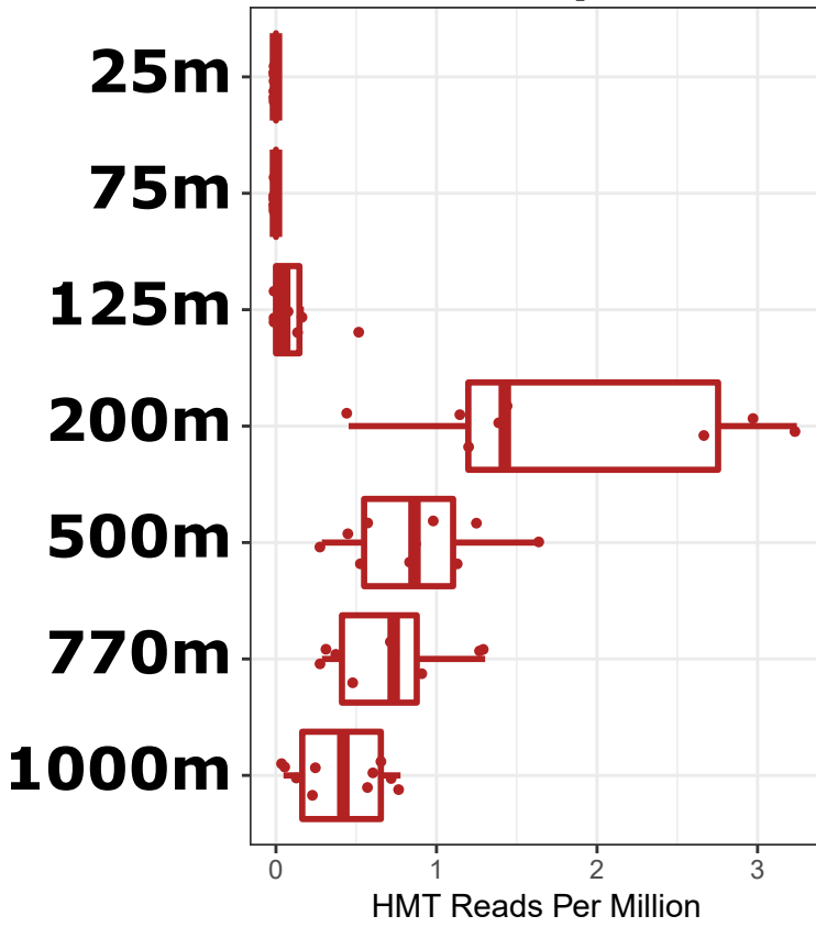
HMT rbcL profile
