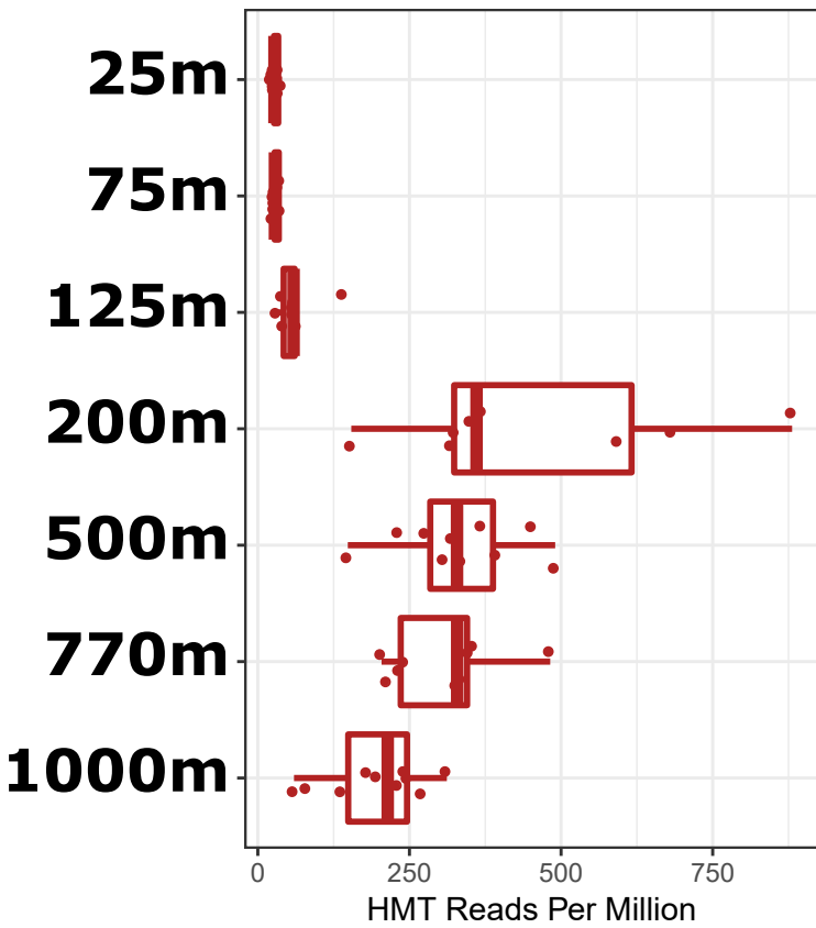
HMT whole genome profile
