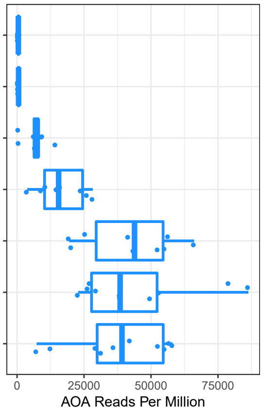
AOA whole genome profile
