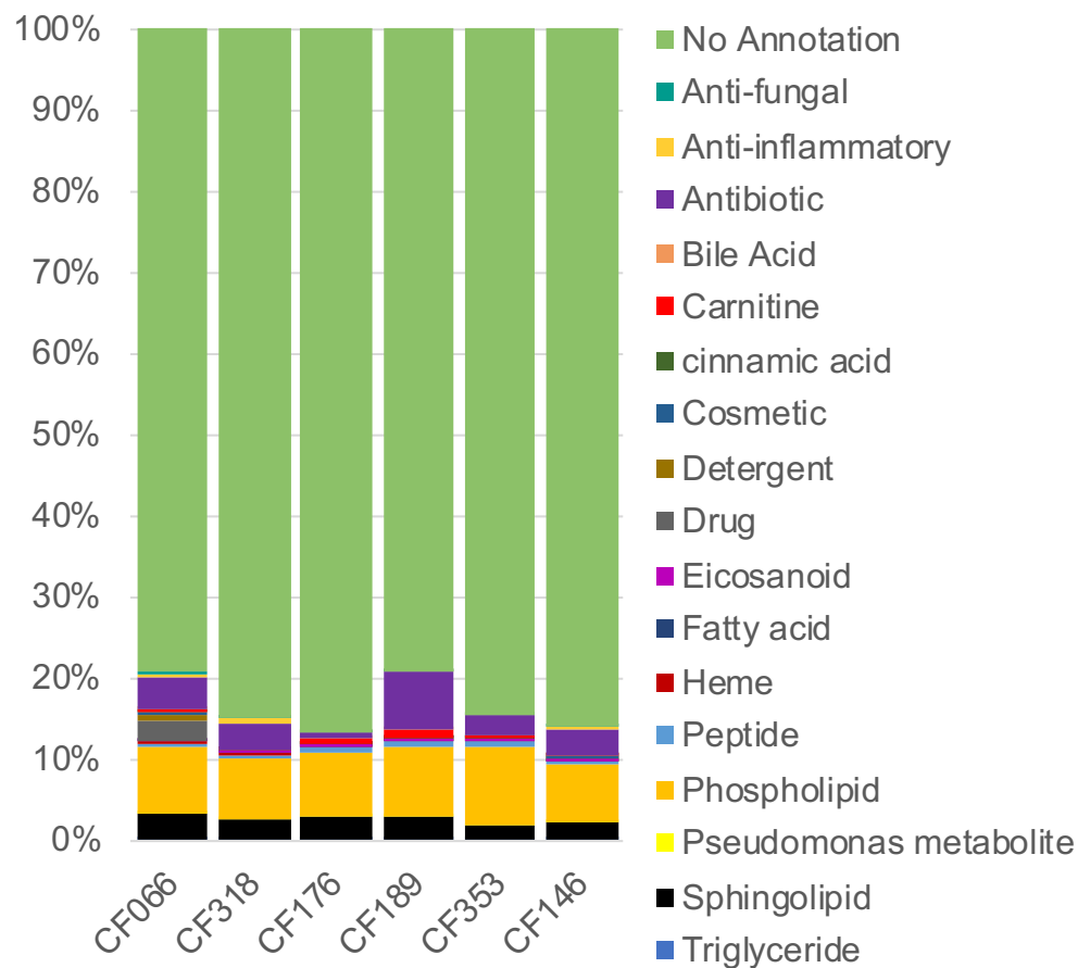
All Mass Spectral Features
