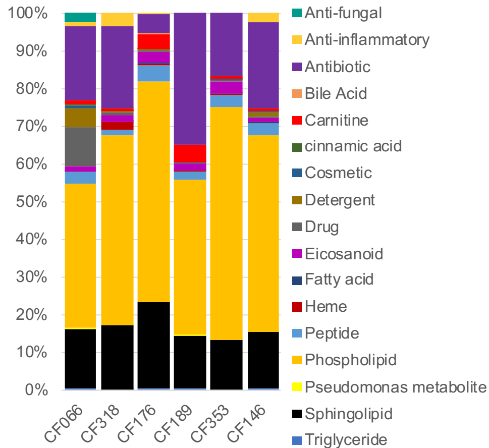
Annotated Mass Spectral Features
