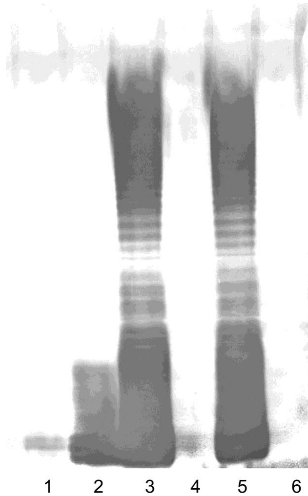
Fig. S1. Lipopolysaccharide (LPS) O-antigen phenotypes of Yersinia strains. Western blot of LPS from 1) Y. pestis KIM6+ wt; 2) Y. pestis KIM6+ ddhD-gmd-pstb ; 3) Y. pseudotuberculosis IP32953 wt; 4) Y. pseudotuberculosis ddhD-gmd:km ; 5) Y. pseudotuberculosis IPmt; and 6) Y. pseudotuberculosis \Delta ddhD-gmd (SY406) grown at room temperature. LPS was extracted and analyzed as described (F. Pouillot et al. , Microbiology 151:3759-3768, 2005).
