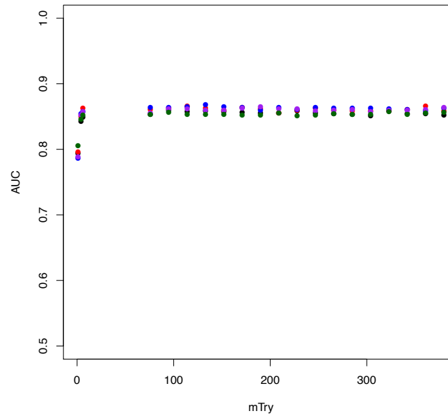
mTry effect on test set
