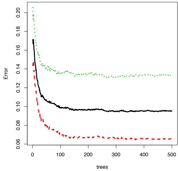
Error rate as a function of nTree
