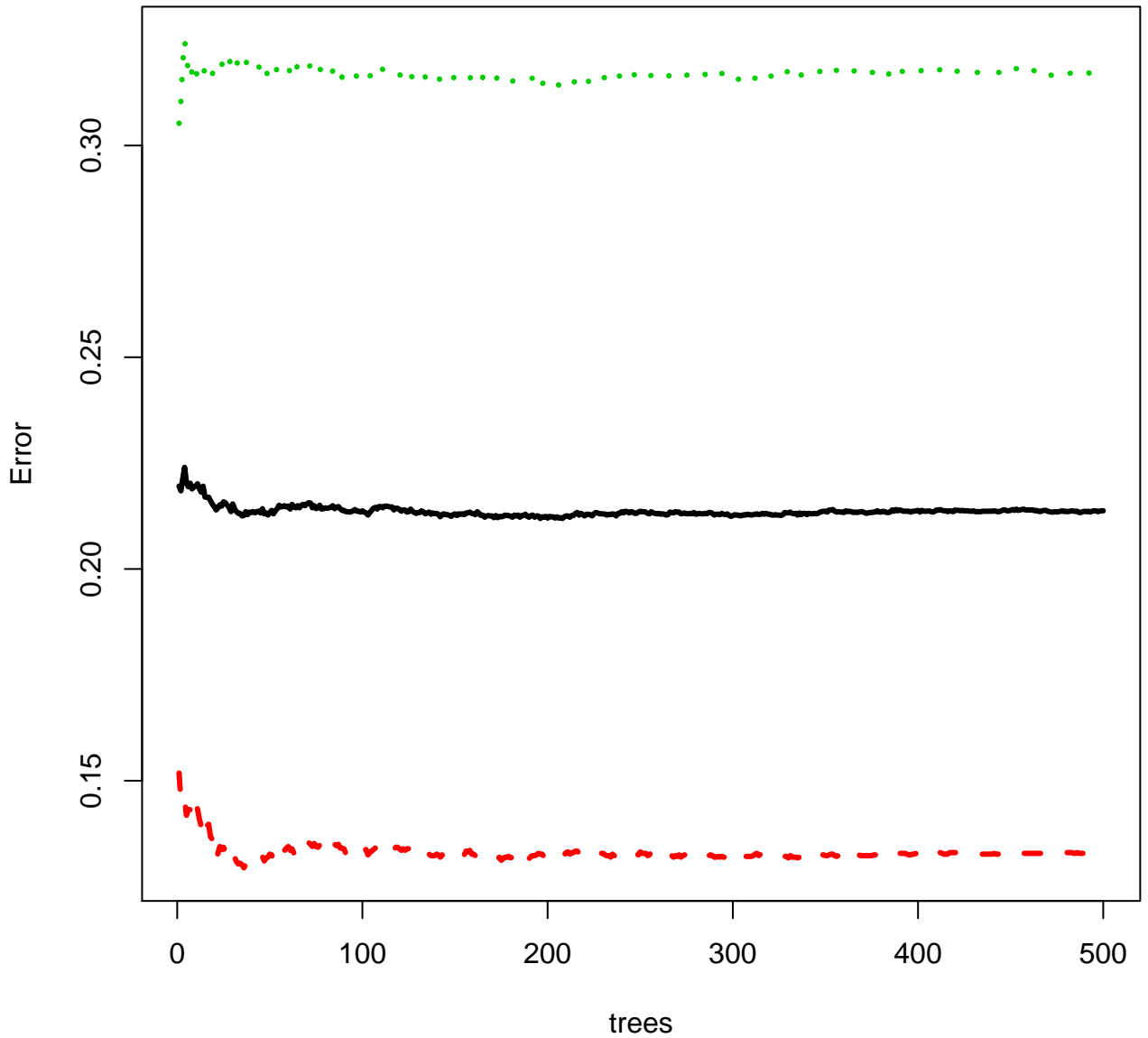
Error rate as a function of nTree
