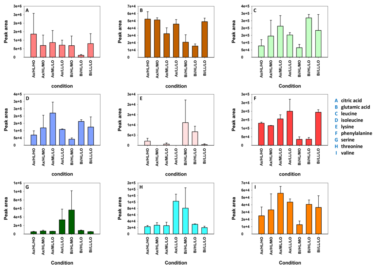
Figure S3. Extracellular metabolite measurements of axenic T. elongatus (Ax) and the binary culture (Bi). Specific turbidostat steady-state conditions are designated with the following abbreviations: high light (1995 \mu\text{mol photons m}^{-2} \text{s}^{-1} ; HL), medium light (1190 \mu\text{mol photons m}^{-2} \text{s}^{-1} ; ML), low light (197 \mu\text{mol photons m}^{-2} \text{s}^{-1} ; LL), high O 2 (pO 2 =0.6 ATM; HO), medium O 2 (pO 2 =0.3 ATM; MO) and low O 2 (pO 2 =0.0 ATM; MO). Measurements are the mean from two biological replicates with standard error.
